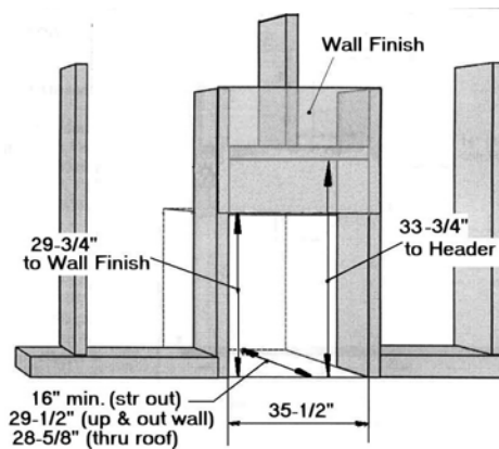
Framing Dimensions
