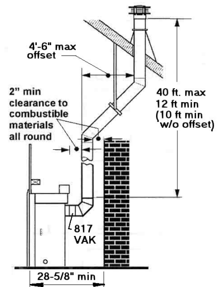
Thru Roof
