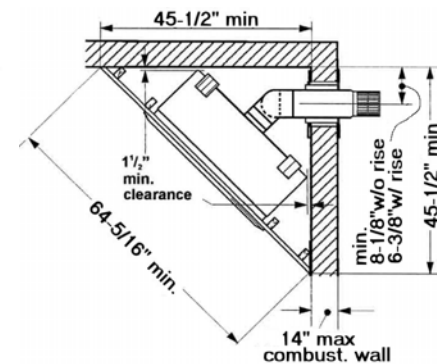
Corner Dimensions
