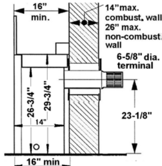
Straight Out
