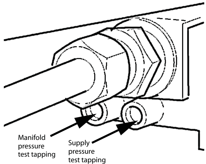
Pressure Testing
