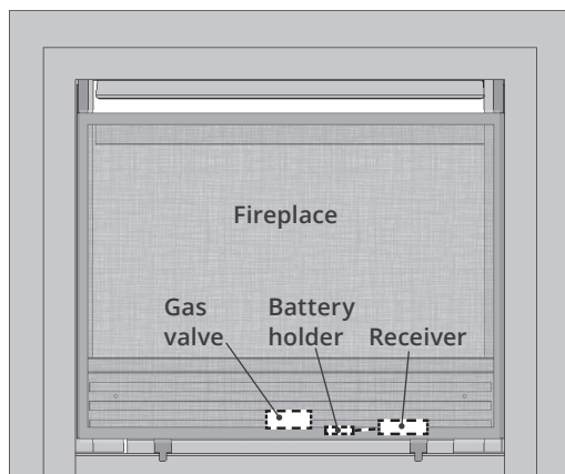
Battery holder located next to receiver on bottom of fireplace behind access panel/fret
