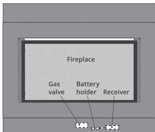
Battery holder located next to receiver on bottom of fireplace behind surround trim
