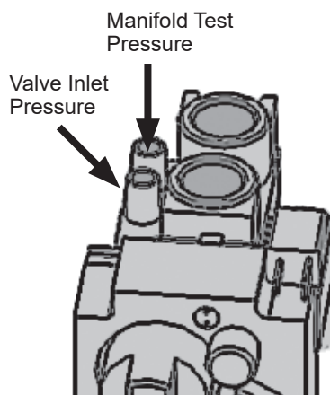
Pressure Testing
